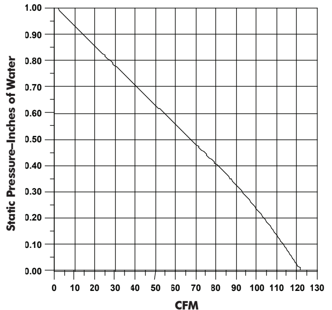
NuVent Product Performance Model NXSS110L
