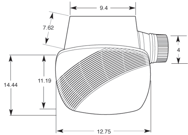
NuVent Product Performance Model NXSS110L
